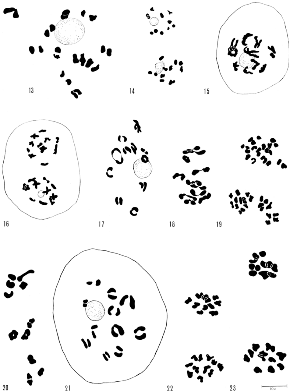
phaeacantha var. major , anaphase I, n = 33 . Fig. 11. O. phaeacantha var. phaeacantha , metaphase II, n = 33 . Fig. 12. O. violacea var. violacea , metaphase II, n = 22 . Fig. 13. Cereus giganteus , diakinesis, n = 11 . Fig. 14. C. greggii var. transmontanus , prophase II, n = 11 . Fig. 15. C. schottii var. australis , diakinesis, n = 11 . Fig. 16. C. schottii var. schottii , prophase II, n = 11 . Fig. 17. C. schottii var. schottii forma monstrosus , diakinesis, n = 11 . Fig. 18. C. thurberi , metaphase I, n = 11 . Fig. 19. Echinocereus engelmannii var. acicularis , telophase I, n = 22 . Fig. 20. E. fendleri var. rectispinus , diakinesis, n = 11 . Fig. 21. Ferocactus acanthodes var. lecontei , diakinesis, n = 11 . Fig. 22. Mammillaria gummifera var. macdougalii , telophase I, n = 11 . Fig. 23. M. wrightii , telophase I, n = 11 .
